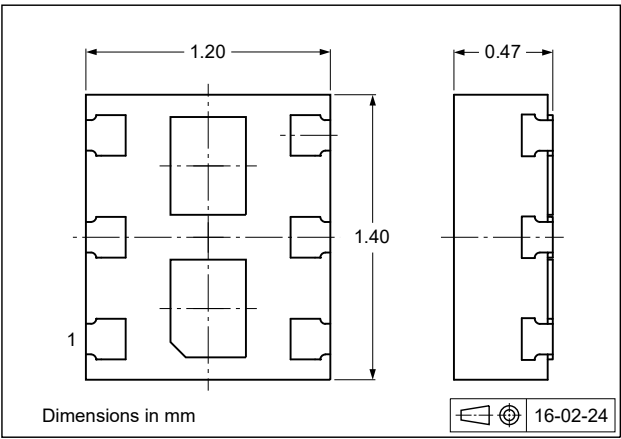
Fig. 19. Package outline DFN1412-6 (SOT1268)
